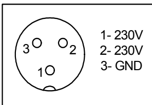
3.1 Alimentation 230VAC
