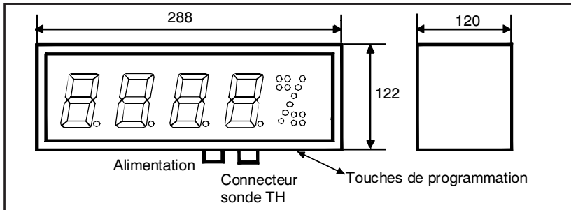
2.1 Dimensions afficheur DN-109TH
