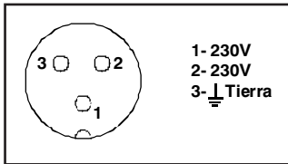
3.1 Alimentation 230VAC
