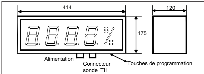
2.2 Dimensions afficheur DN-119TH
