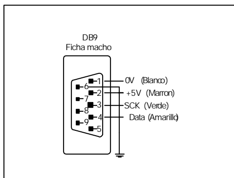
CONECTOR SERIE DN-109TH, DN-119TH y DN-129TH
